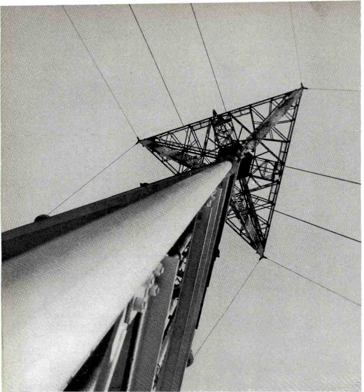
World's first 3-antenna, candelabra-type TV tower built for Baltimore stations WBAL, WJZ and WMAR. Tower Design and Fabrication: Dresser-Ideco Company, Columbus, Ohio. Tower Erector: J. F. Beasley Construction Company, Muskogee, Oklahoma.
